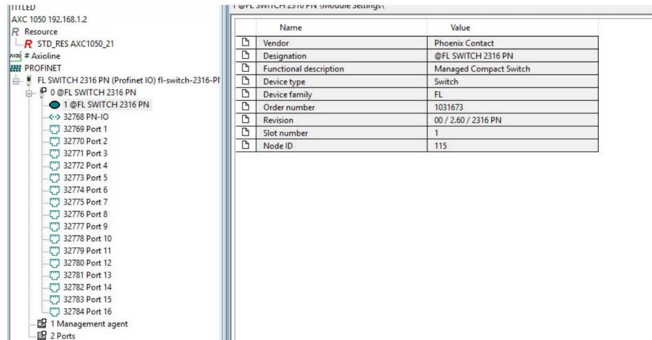
Figure 4-1 Device details
